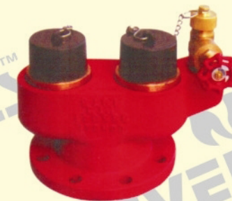
Two Way Fire Brigade Inlet
